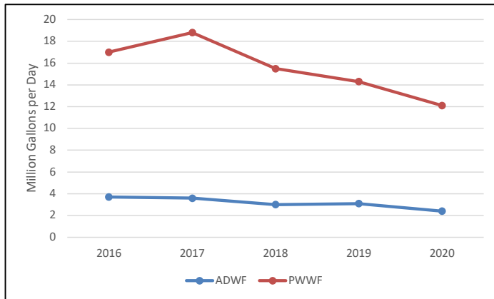
Figure 7-3: WBSD Wastewater Flows, 2016-2020
