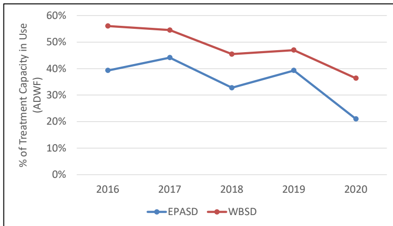
Figure 7-5: Wastewater Treatment Capacity in Use, 2016-2020
