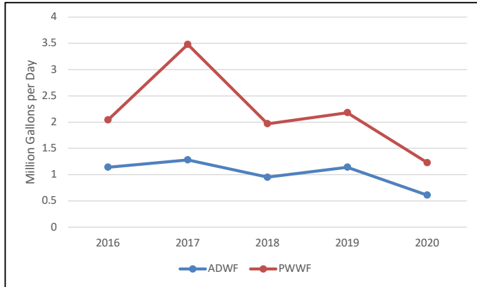
Figure 7-4: EPASD Wastewater Flows, 2016-2020
